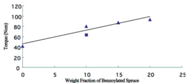
Figure 3 Effect of weight fraction of benzoylated spruce TMP on the torque observed after 8 min melt mixing; \blacktriangle benzoylated spruce TMP-poly(styrene) composites; \blacksquare spruce TMP-poly(styrene) composite (values recorded after 8 min of melt mixing). [Color figure can be viewed in the online issue, which is available at www.interscience.wiley.com .]
