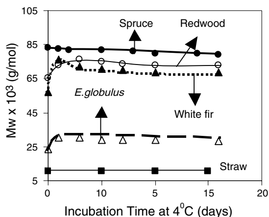
Fig. 4. Effects of incubation at 4 °C on the apparent weight-average molecular weight ( M_w ) of lignins isolated from spruce (black-filled circles), redwood (open circles), white fir (black-filled triangles), E. globulus (open triangles) and straw (black-filled squares). All the lignins were previously completely acetobrominated.
